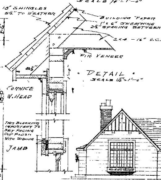
ELEVATION SCALE 1/4" = 1'-0"
