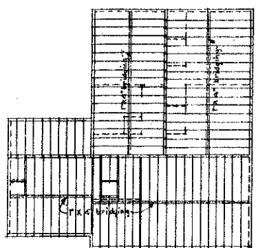
FRAMING PLAN
