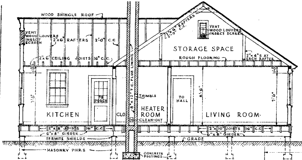
CROSS SECTION ON LINE "A-A"
