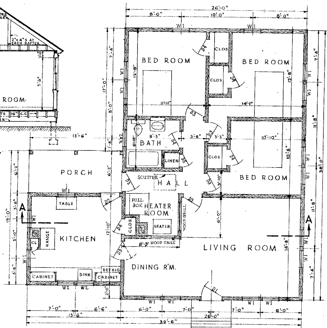
FLOOR PLAN
