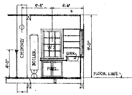
SECTIONS THRU KITCHEN
