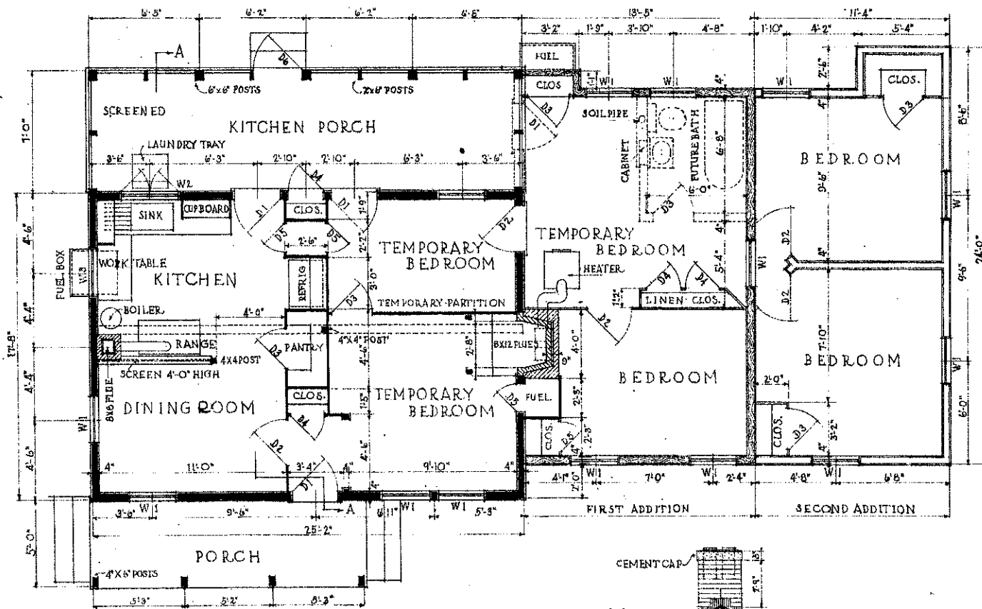
ORIGINAL PLAN SCALE 1/4" = 1'-0"
