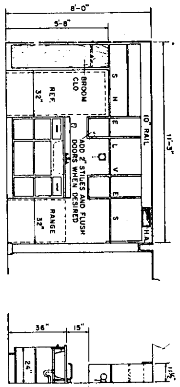
KITCHEN CABINETS SCALE - 1/8" = 1'-0"
