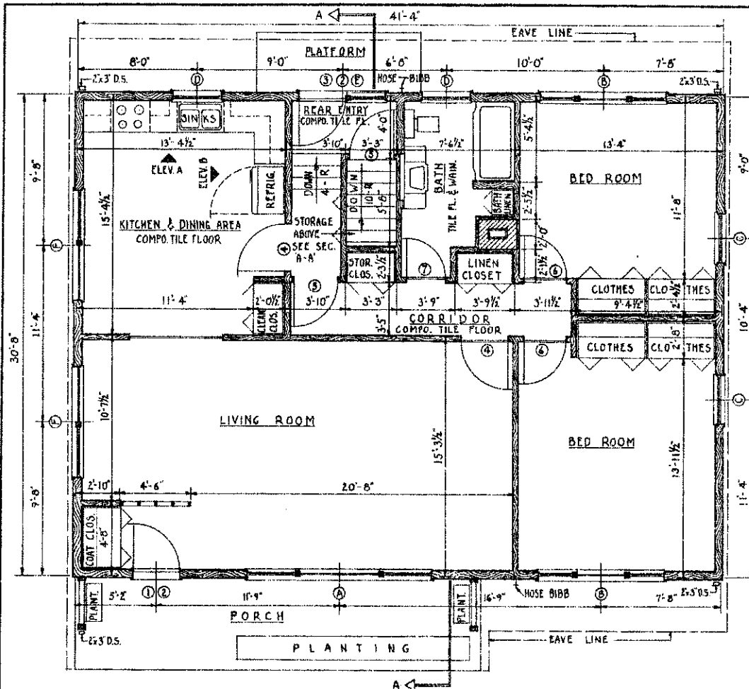
FIRST-FLOOR PLAN
