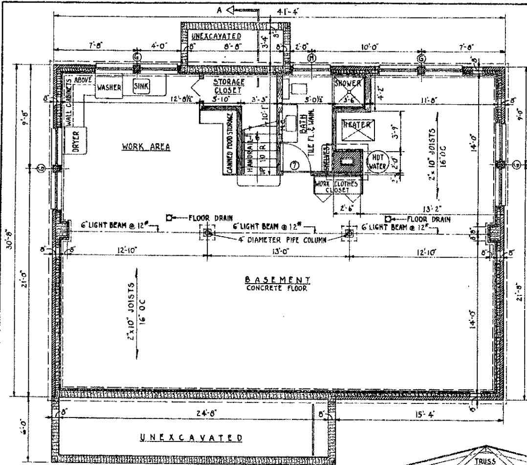
BASEMENT FLOOR PLAN SHOWING FOUNDATIONS SCALE 1/4" = 1'-0"
