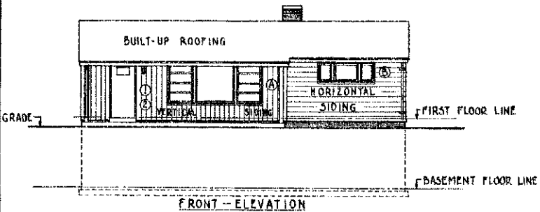
ELEVATIONS SCALE 1/2"=1'-0"
