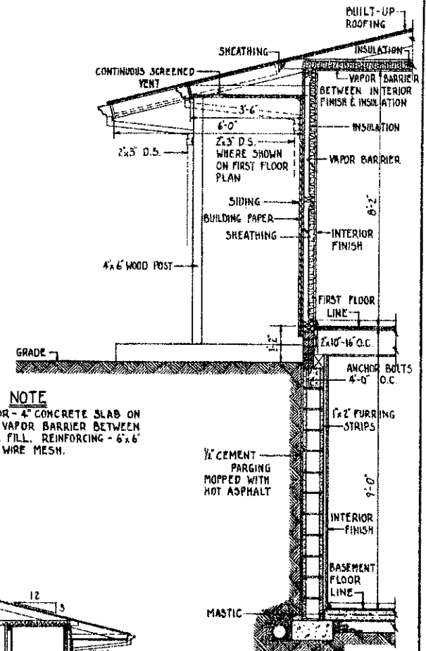
TYPICAL WALL SECTION SCALE 1/2" = 1'-0" SHOWING TYPICAL OVERHANG - AND WIDE OVERHANG AT FRONT ENTRANCE
